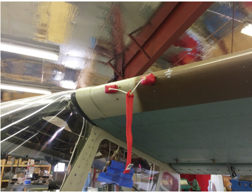
Siai Marchetti 1019 Ventilation Scoop Plugs ENGINE PLUGS PREVENT BIRD NEST FOD. Piper Saratoga Engine Cowling Bird's Nest
