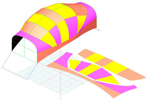
Aquila A210 Canopy Cover, 3D model
