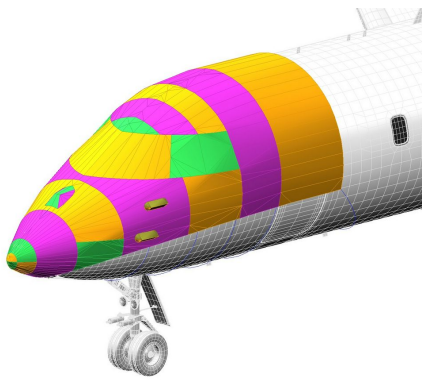
Bombardier Global Express Cockpit/Nose Cover, 3D model
