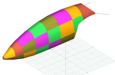
Rolladen-Schneider LS-4 Canopy/Nose Cover
